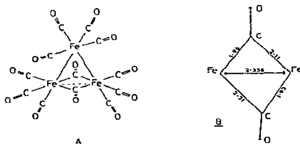
Fig. 6. A, Molecular structure of \text{Fe}_3(\mu\text{-CO})_2(\text{CO})_{10} (compound 28). B, Details of the carbonyl bridge system (planar projection, drawn to scale).
