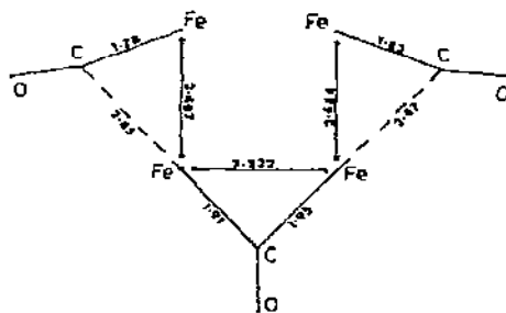
Fig. 14. Details of the \mu_2 carbonyl bridge system in the [\text{Fe}_4(\mu\text{-CO})_4(\text{CO})_9]^{2-} anion (compound 42). (Drawn to scale.)
