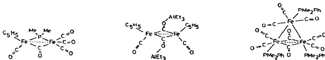
Fig. 3. Molecular structure of Fe_2(\mu-CO)(\mu-PMe_2)(CO)_4(C_5H_5)_2 (compound 20).
