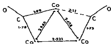
Fig. 19. Details of the \mu_2 carbonyl system in \text{Co}_3(\mu\text{-CO})_3(\text{C}_5\text{H}_5)_3 (compound 67). (Drawn to scale.)
