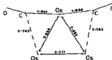
Fig. 22. Details of the carbonyl bridge system in V_2(\mu\text{-CO})_2(\text{CO})_3(\text{C}_5\text{H}_5)_2 (compound 95). (Planar projection, drawn to scale.)
