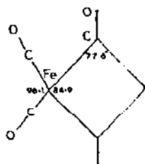
Fig. 32. Molecular structure of \text{Pd}_2(\mu\text{-CO})(\mu\text{-dam})_2\text{Cl}_2 (compound 111). (Phenyl groups omitted for clarity.)
